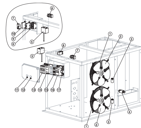
ELECTRIC PARTS
