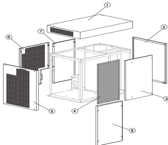
SHELL ASSY
