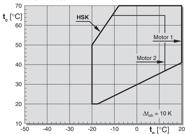
R134a CR 100%
