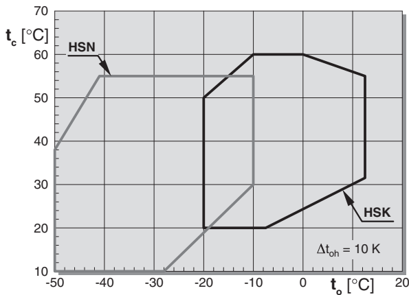
R22 CR 100%
